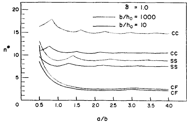
Fig. 3. Buckling coefficient, n^* = \sigma_x h_0 b^2 / D_0 \pi^2 of Mindlin plate with tapered thickness subjected to the uniform compressive load, \sigma_x ; ( \nu = 0.3 , \delta = 1.0 ).
